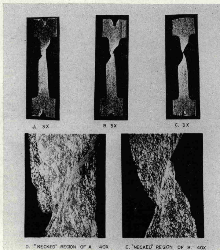
FIG. 12. Gliding type of fracturing at high pressures 175°C.
